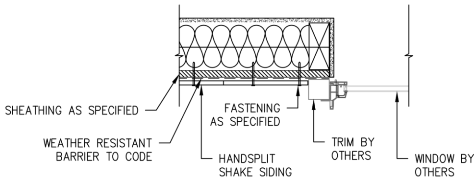
C 3 HANDSPLIT SHAKES WINDOW JAMB SECTION NOT-TO-SCALE
