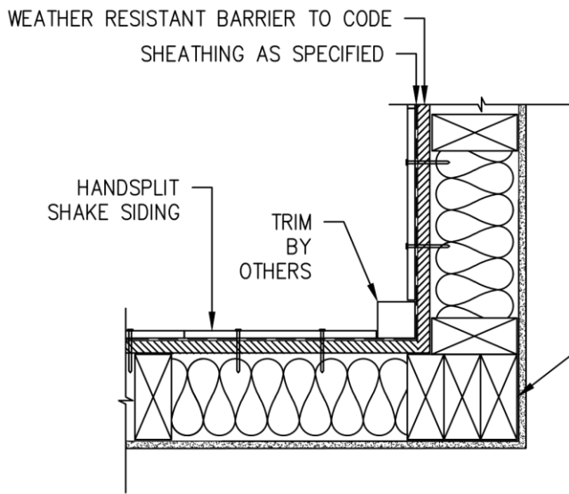
B 6 HANDSPLIT SHAKES INSIDE CORNER DETAIL PLAN VIEW NOT-TO-SCALE
