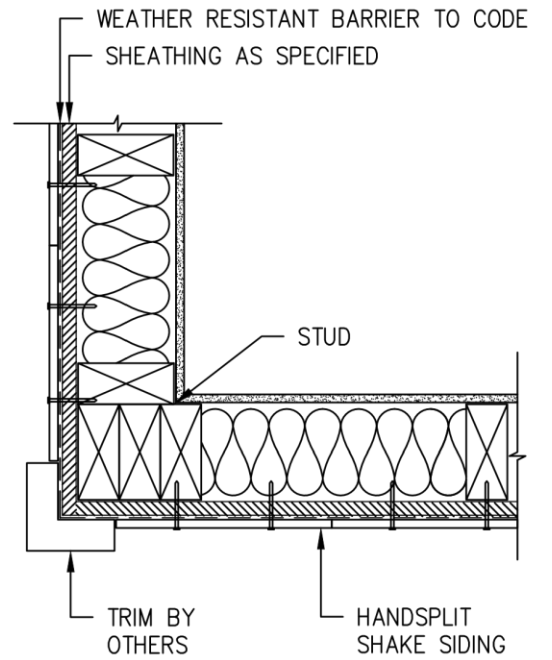
A 6 HANDSPLIT SHAKES OUTSIDE CORNER DETAIL PLAN VIEW NOT-TO-SCALE
