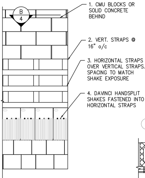
A 4 HANDSPLIT SHAKES OVER CMU OR CONCRETE WALL ELEVATION VIEW NOT-TO-SCALE
