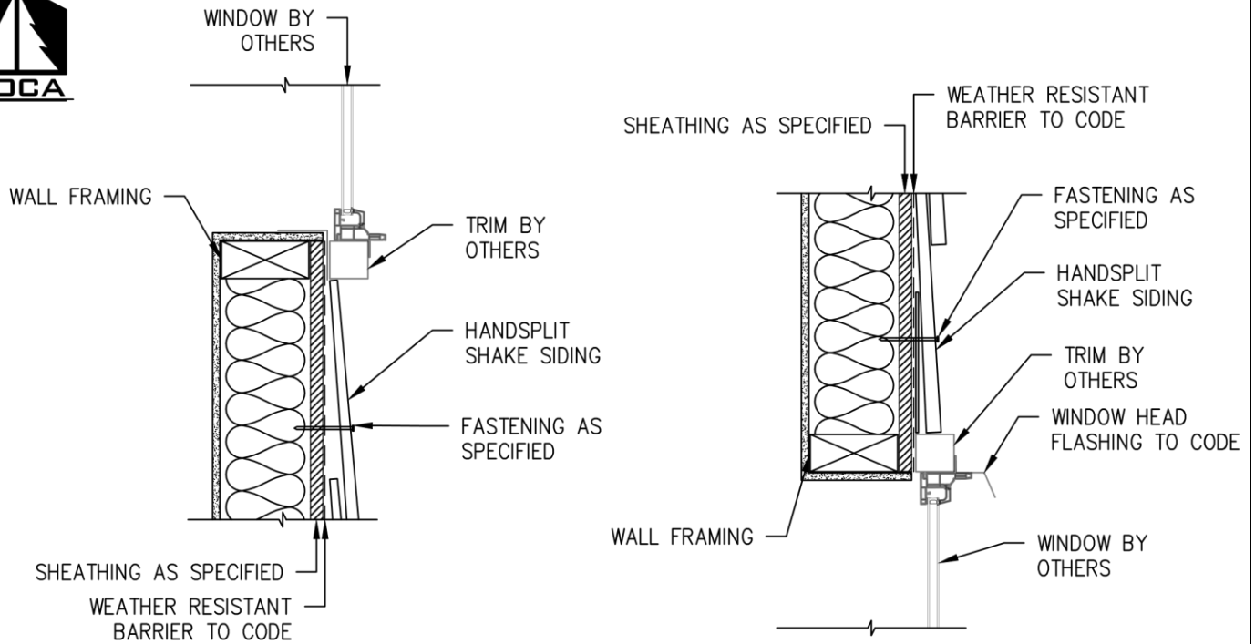
A 3 HANDSPLIT SHAKES WINDOW SILL SECTION NOT-TO-SCALE
